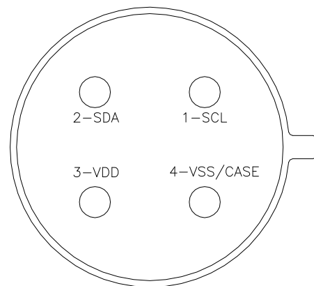
Figure 4. Package Top View
